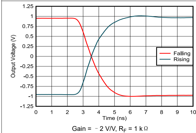
图 7-17. Settling Time
