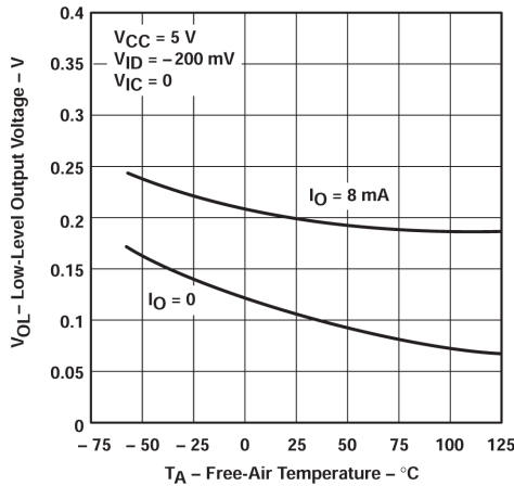
图 5-9. Low-level Output Voltage vs Free-air Temperature
