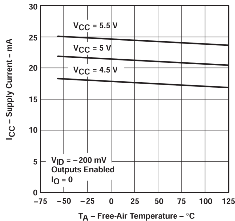
图 5-13. Supply Current vs Free-air Temperature
