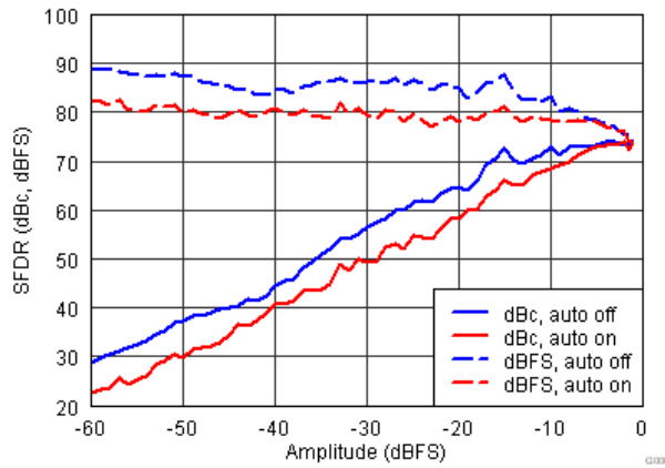
图 15. SFDR vs Amplitude (f in = 230 MHz)
